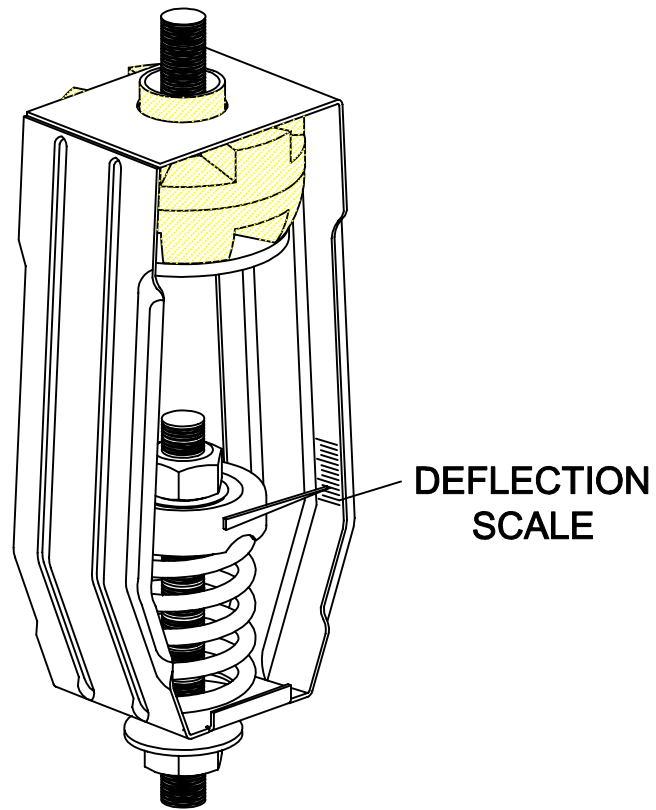
SRPH PRECOMPRESSED SPRING HANGER ASHRAE TYPE 3
