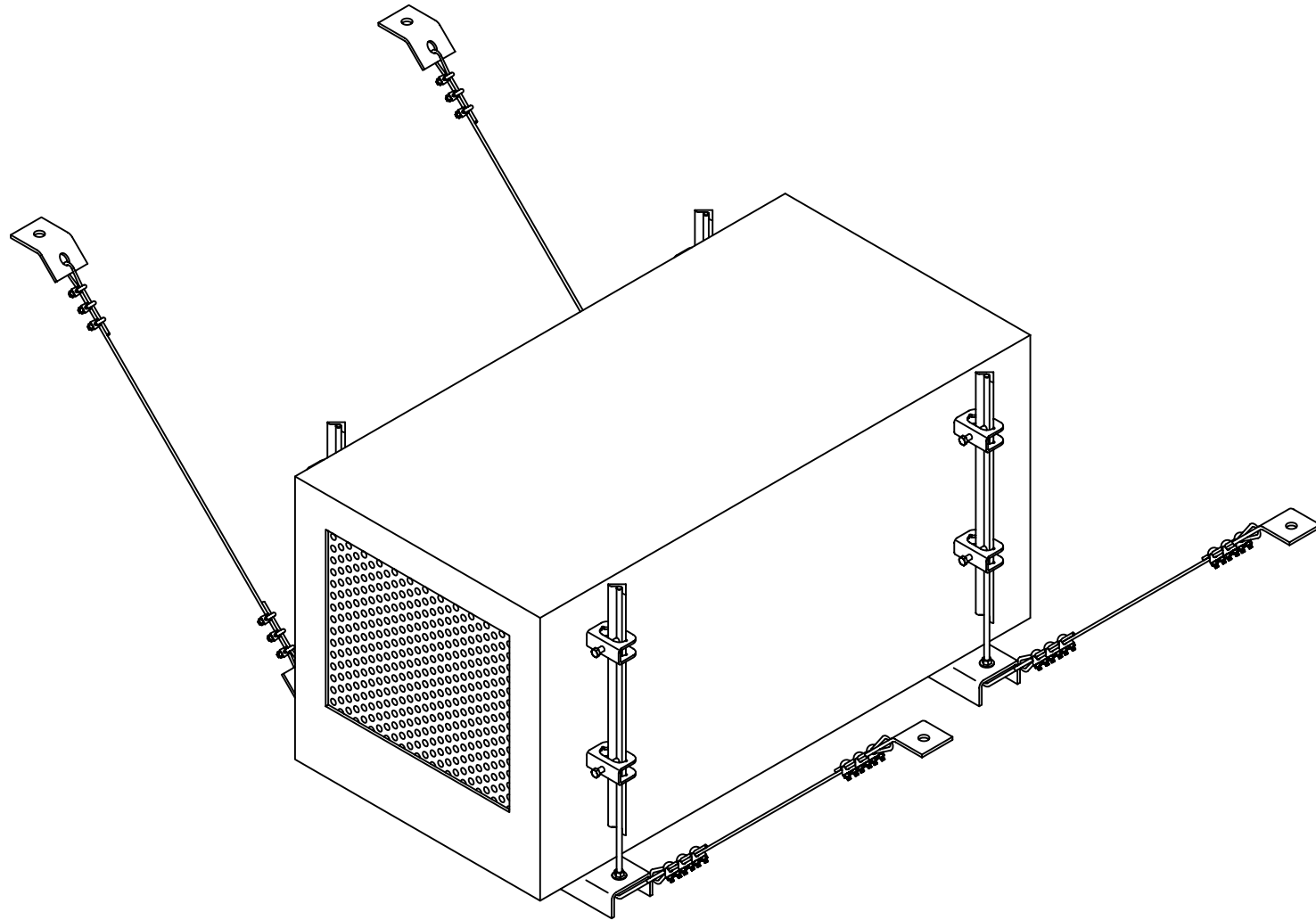
KINETICS MODEL KSCC BULK CABLE RESTRAINT KIT WITH KHRC ROD STIFFENER CLAMPS ASHRAE TYPE J
