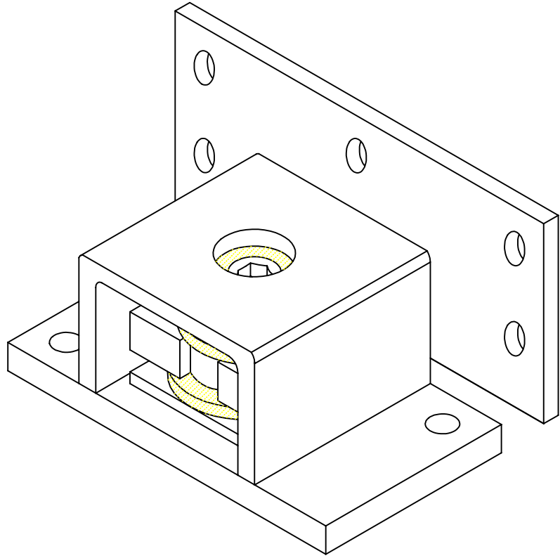
FMS RESTRAINT ALL DIRECTIONAL SNUBBER
