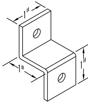
ENLARGED VIEW OF MOUNTING BRACKET
